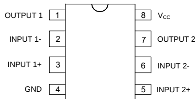
(DIP-8/TDIP-8)
